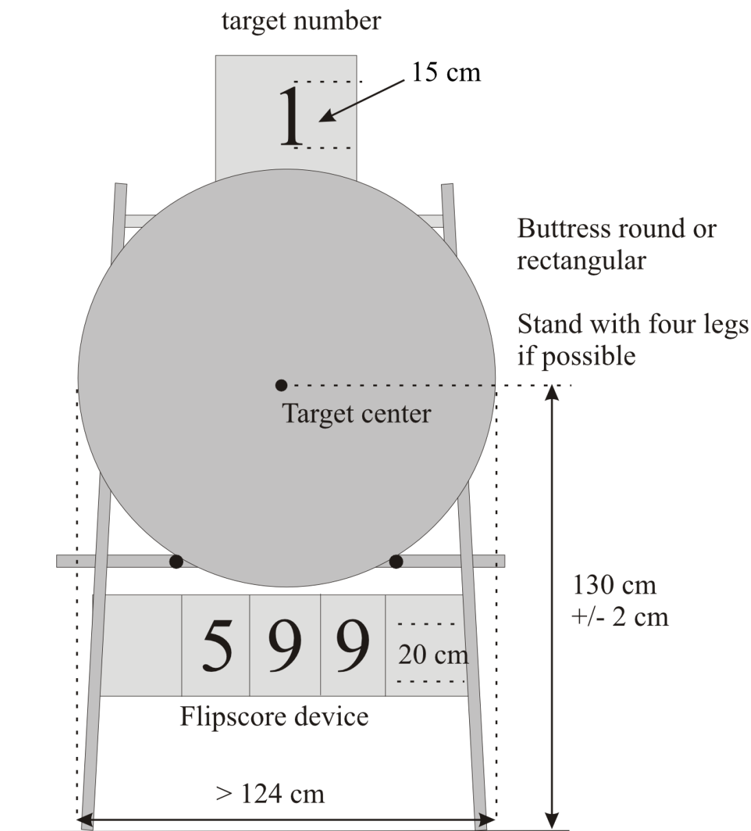
Image 4: Indoor target butt set-up
